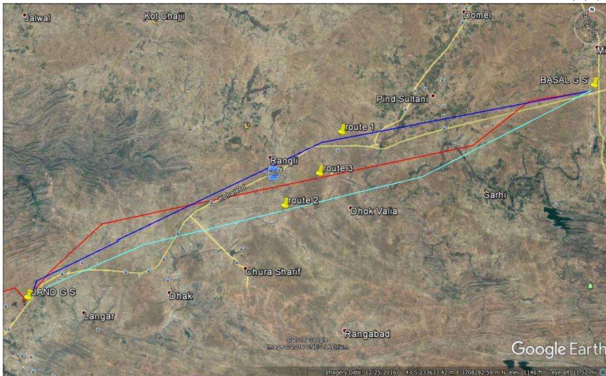
Figure 4.1: Proposed 132 kV Basal – Jand Transmission Line alongwith Alternative Route (Route 3 in red colour is selected as suitable route).
