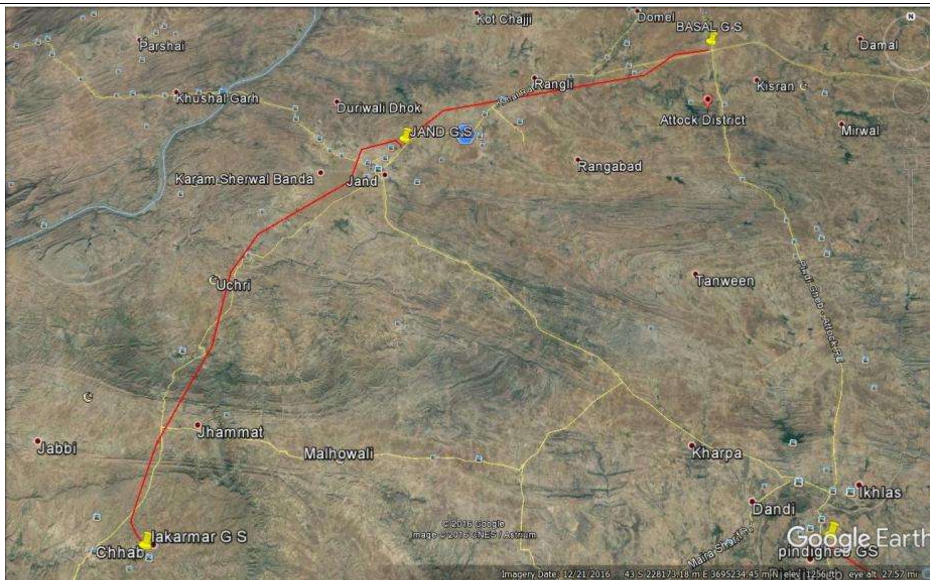
Figure 3.2: Proposed 132 kV Basal – Jand Transmission Line on Google Map.
