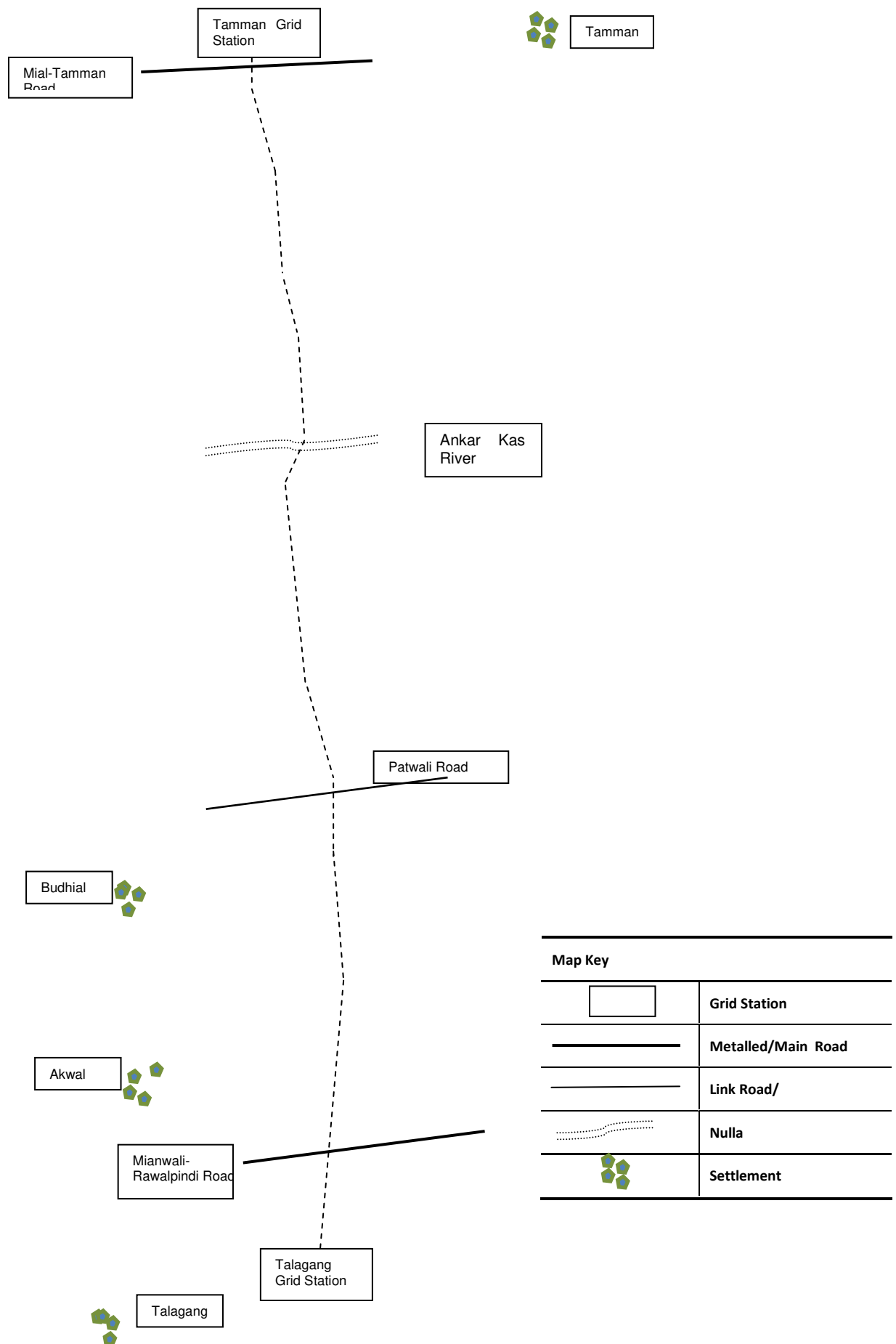
Figure: 1 Schematic Map/Sketch of 132 KV feeding T/line of Tamman G/Station
